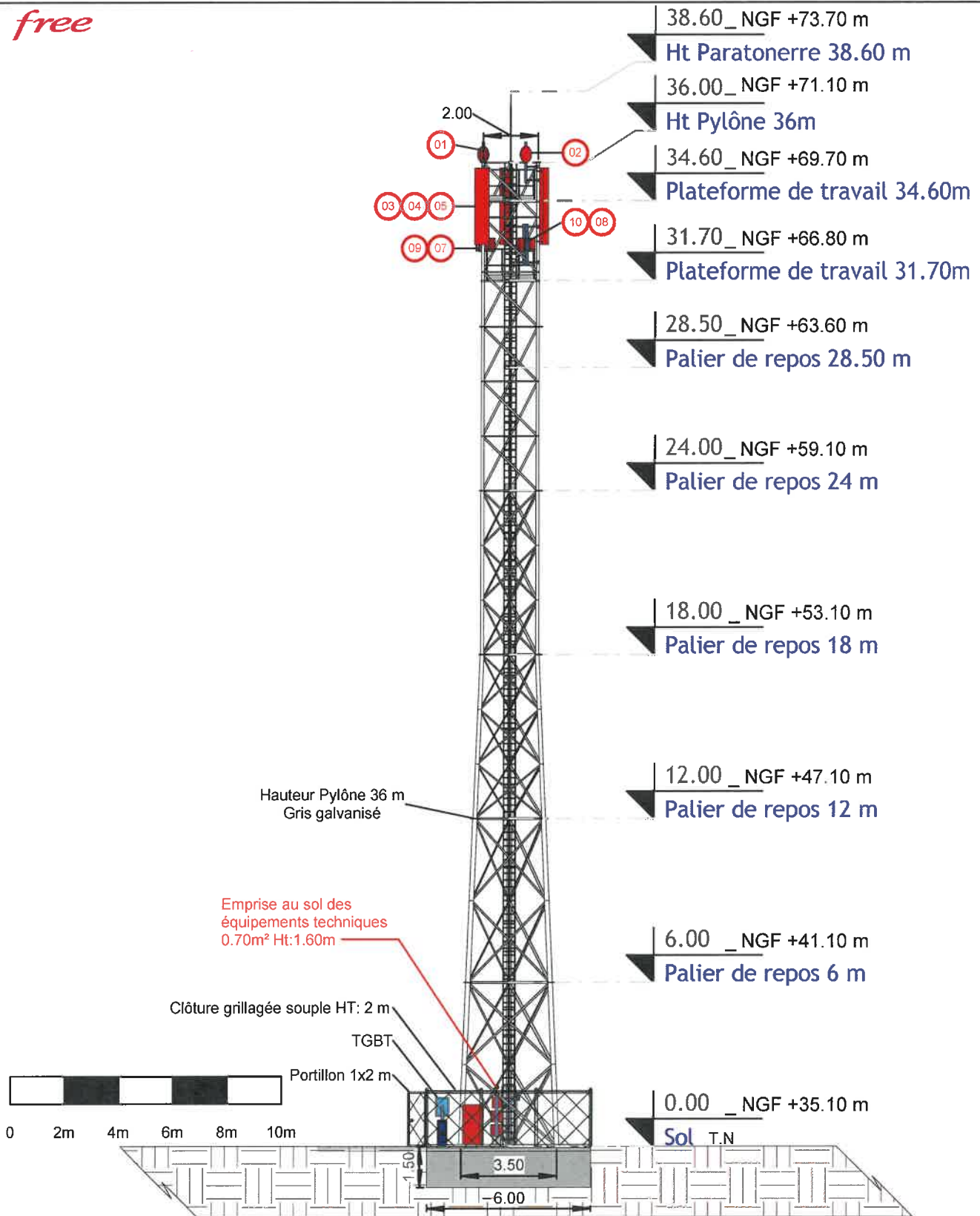
FREE-Elévation Sud-Pylône-Pose
